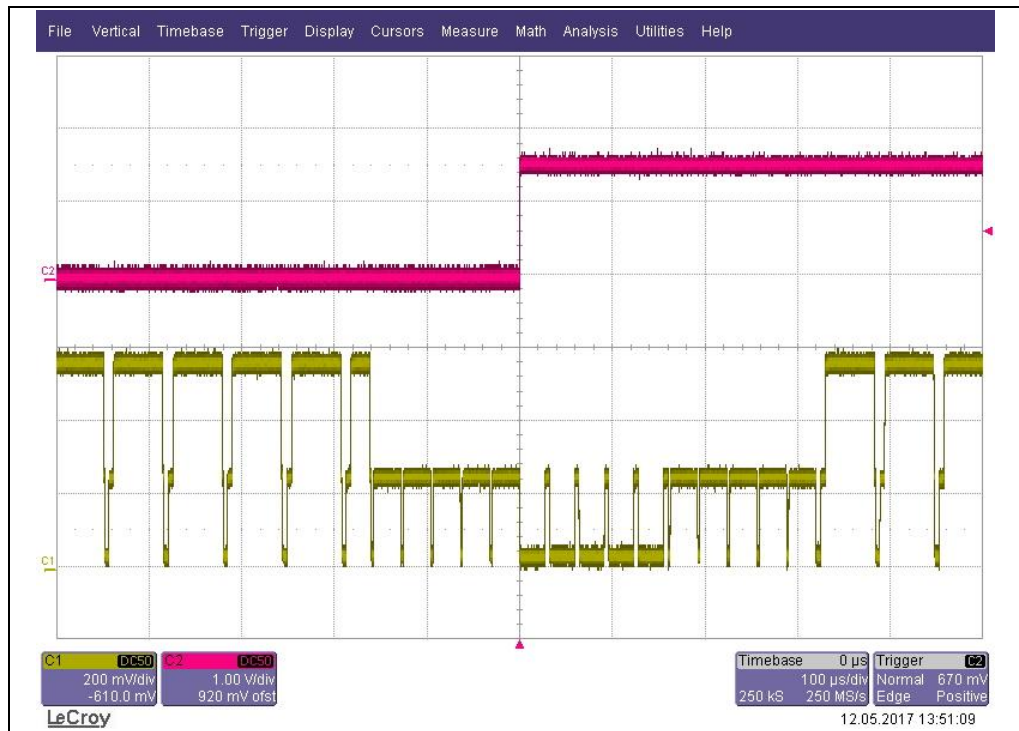
Figure 6 Analog Video Mode 625i (master operation)
