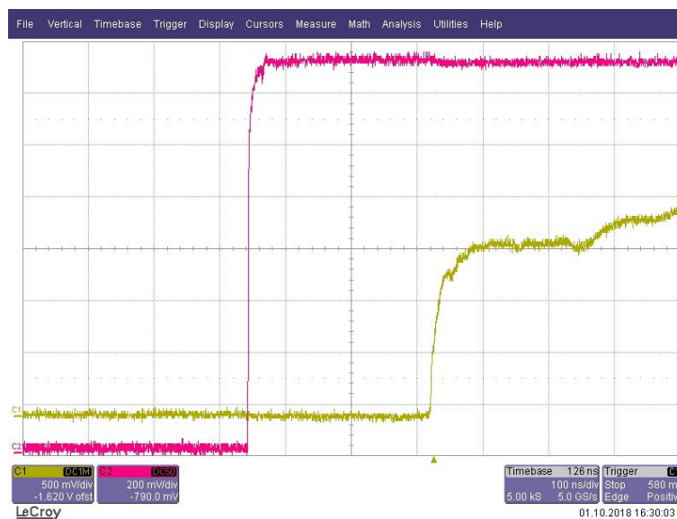
figure 1. 1PPS measurement
