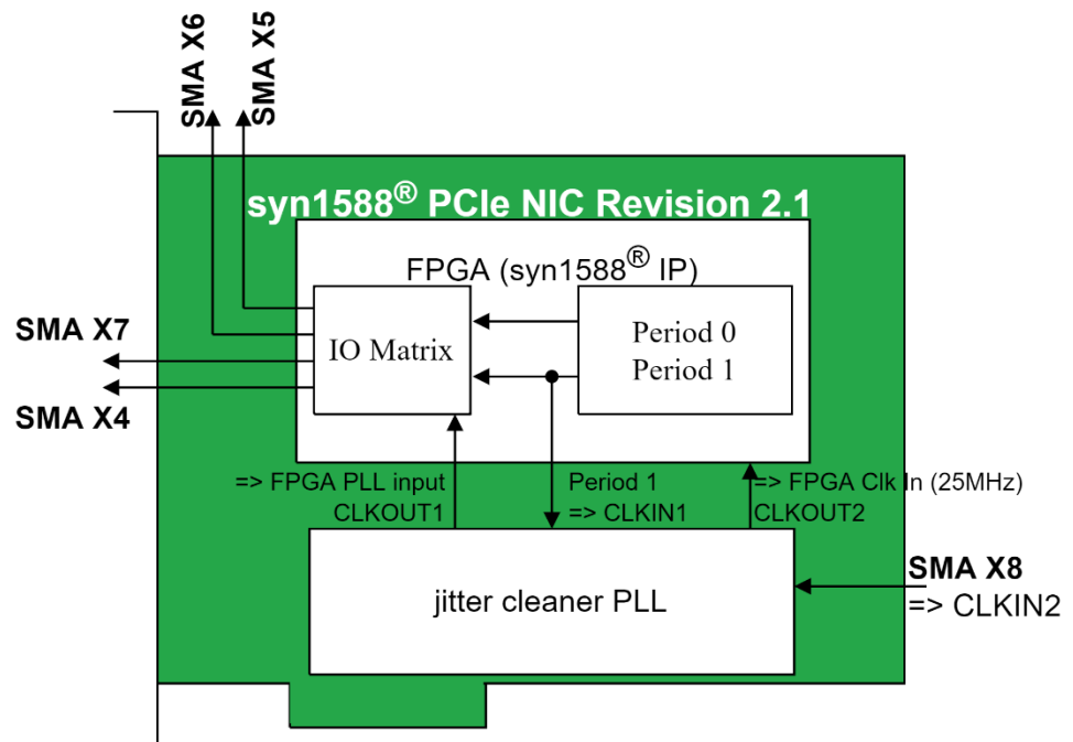
Figure 4: syn1588 ® PCIe NIC Rev 2.1 SMA connectors
