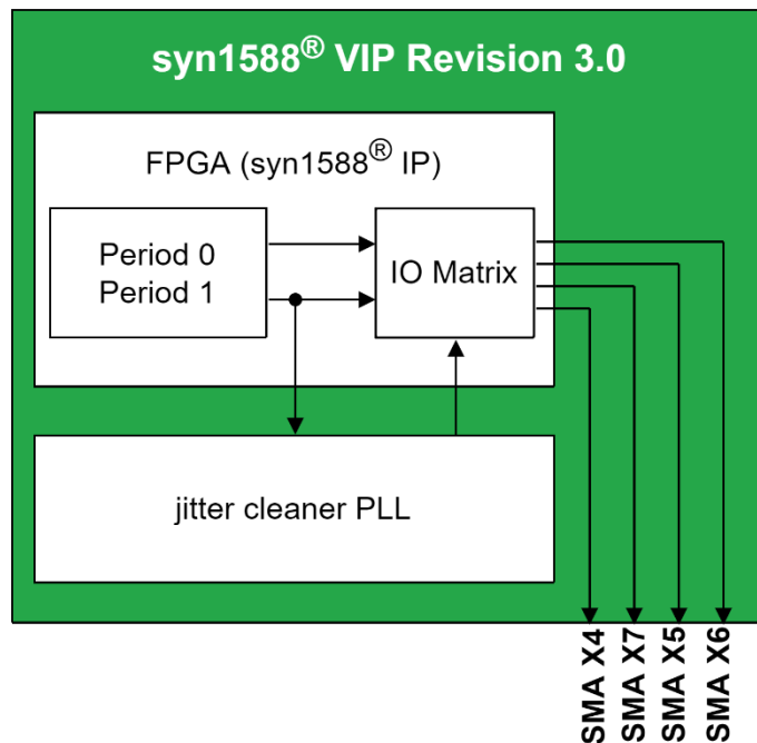
Figure 6: syn1588 ® VIP Evaluation Board Revision 3.0 SMA connectors
