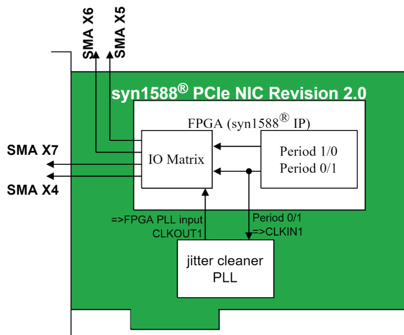
Figure 3: syn1588 ® PCIe NIC Rev 2.0 SMA connectors
