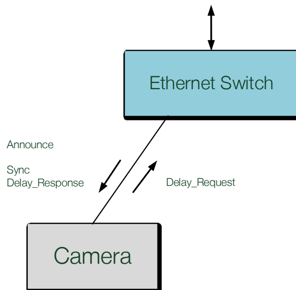
Figure 4: PTP: communication
