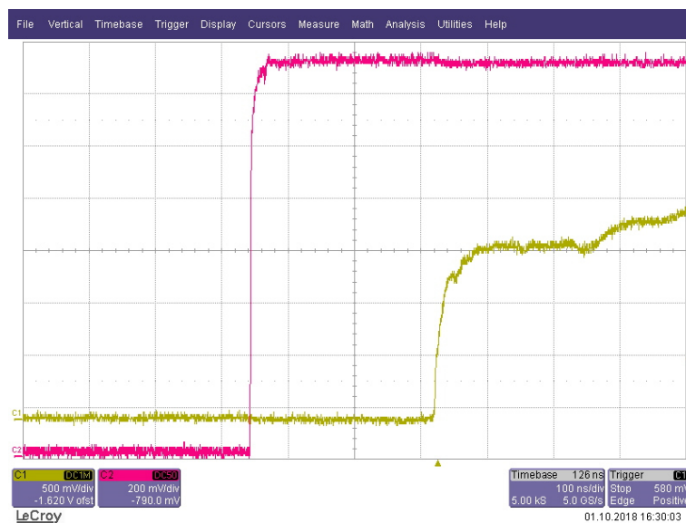
figure 1. 1PPS measurement
